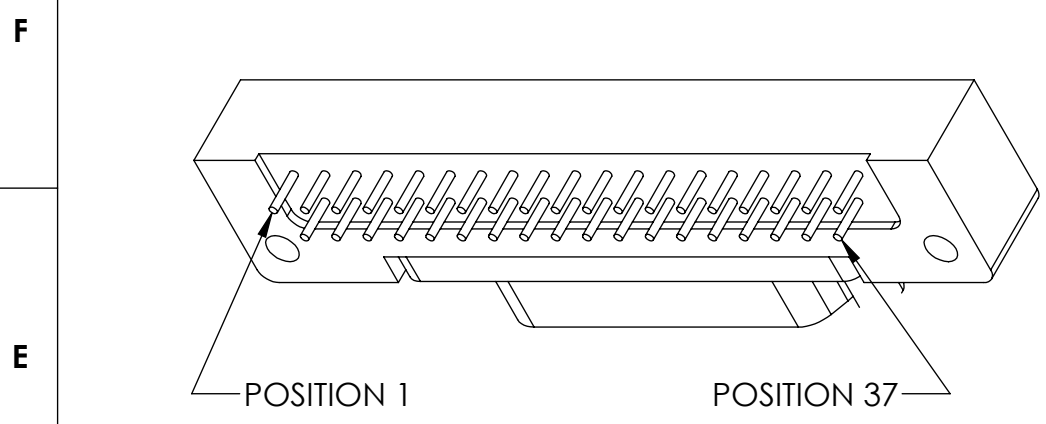
PCB VIEW
