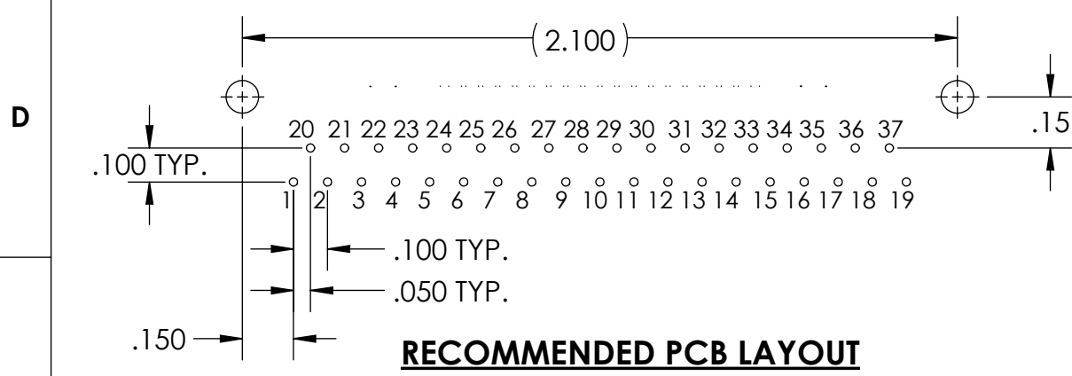
PCB VIEW
