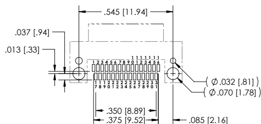
SIZE 31 - VIEW A
