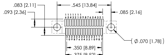
SIZE 31 - VIEW A
