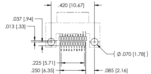
SIZE 21 - VIEW A
