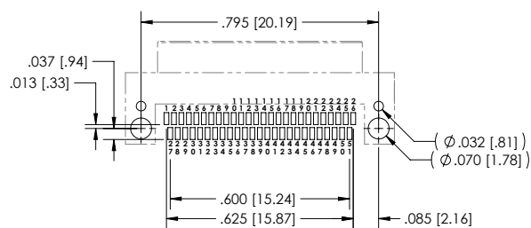
SIZE 51 - VIEW A
