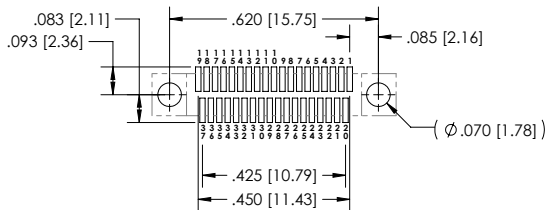
SIZE 37 - VIEW A
