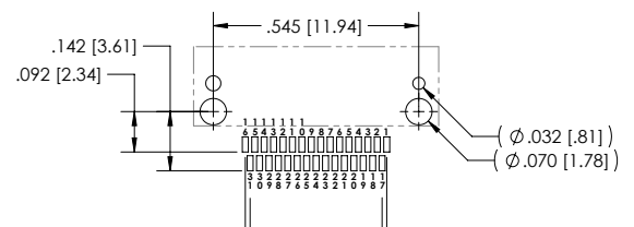
SIZE 31 - VIEW A
