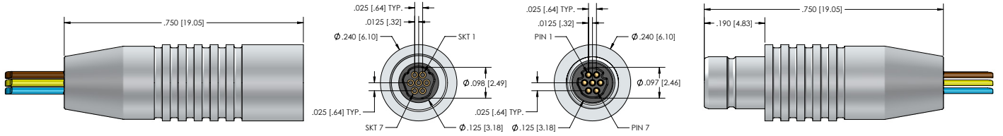
7 POSITION RECEPTACLE
