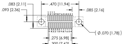
SIZE 25 - VIEW A
