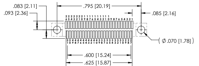
SIZE 51 - VIEW A
