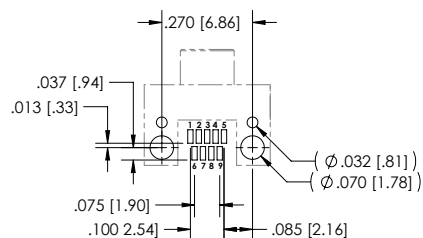
SIZE 9 - VIEW A
